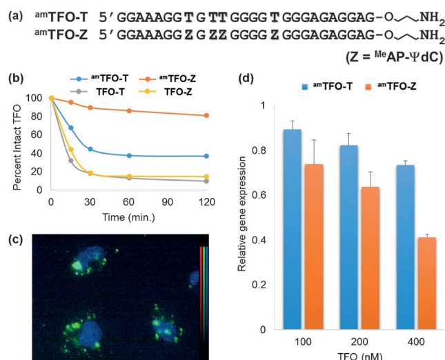
Figure 3. a) The sequences of the aminopropyl-modified TFOs. b) Evaluation of amTFO-T and amTFO-Z against exonuclease I digestion. Each TFO was treated with exonuclease I (0.5 U) in a buffer containing 20 mM Tris-HCl (pH 7.5), 2.5 mM MgCl 2 , and 2.5 mM spermidine at 37°C for 0–120 min. The digestion was analyzed on a 15% denaturing polyacrylamide gel. c) Confirmation of the endogenous uptake of TFO by fluorescence microscopy. The green represents the FITC-labeled amTFO-Z, and the blue indicates nuclear staining with Hoechst 33258. d) Intracellular inhibition of hTERT gene expression using amTFO-T and amTFO-Z. The relative gene expression levels were obtained by normalizing the amount of hTERT mRNA with GAPDH mRNA. The standard deviations were calculated from three independent experiments.
